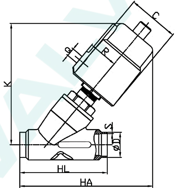
Welded Connection
